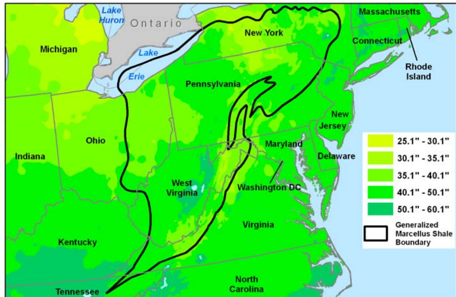
Figure 8: Average Annual Rainfall in the Area of the Marcellus Shale Play Source: NOAA
